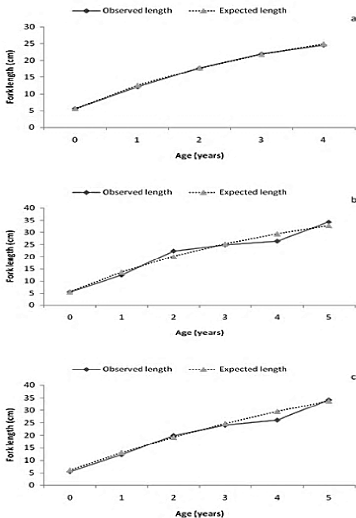
Figure 2: Observed lengths at age data and expected von Bertalanffy growth curves for males plus unsexed (a) females plus unsexed (b) and whole samples (c) of Capoeta damascina from Gheslugh Reservoir.
